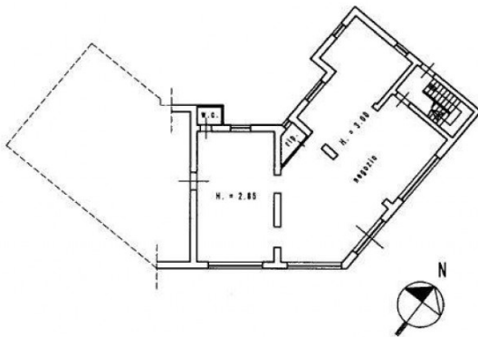
PIANO TERRENO
