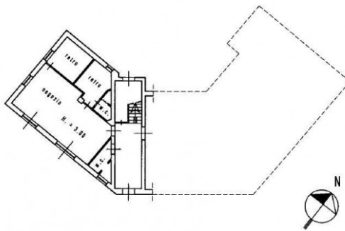
PIANO TERRENO
